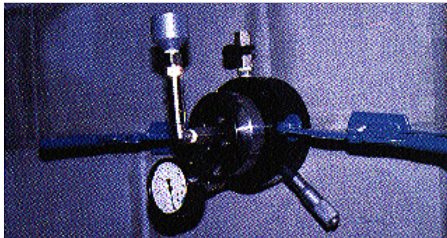
Permeability testing devices measure the time for a known amount of water to be forced into the masonry at a preset pressure. The shorter the time period, the more permeable the masonry.
