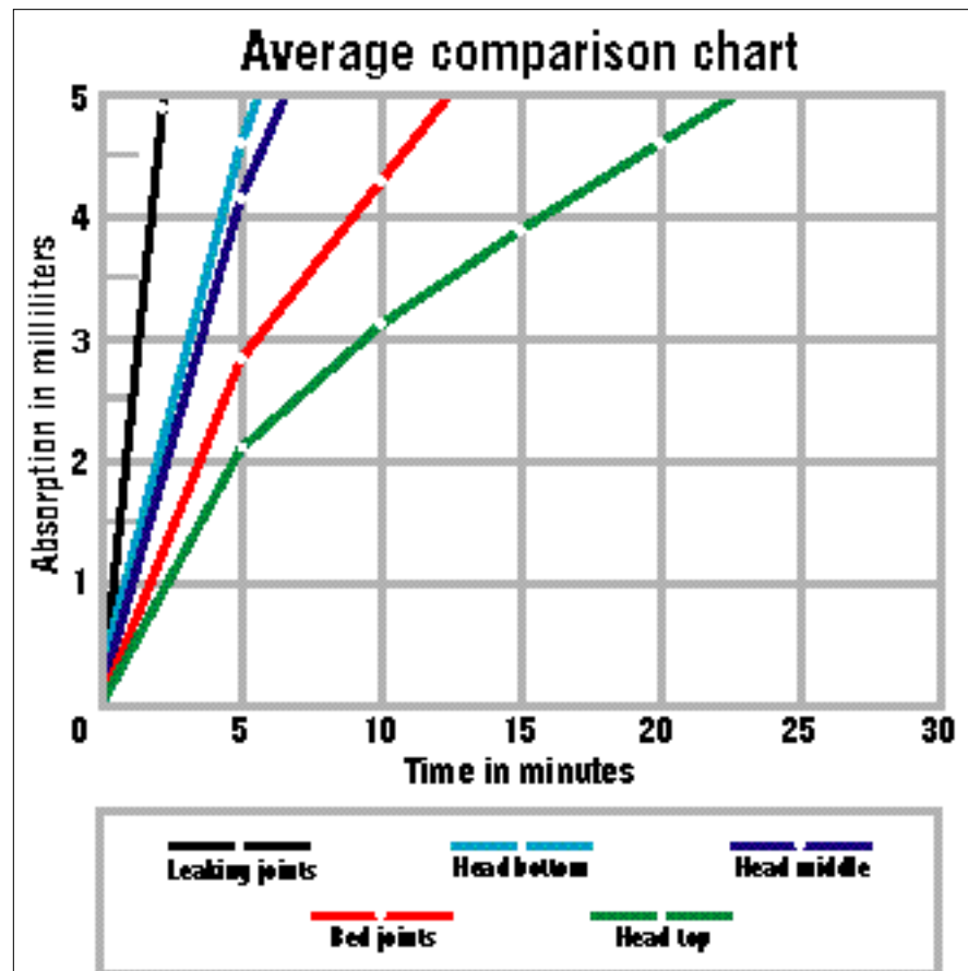
Figure 2. Absorption graphs show the volume of water absorbed in milliliters versus time. The more permeable the masonry, the faster 5 ml of water will be absorbed.
